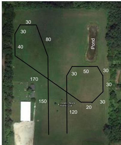
Saturday - 810 yards
