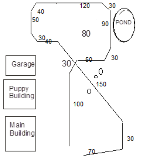
Sunday – 860 yards
